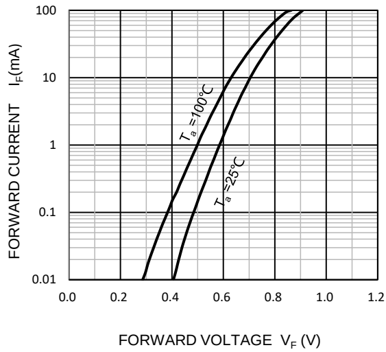
Forward Characteristics
