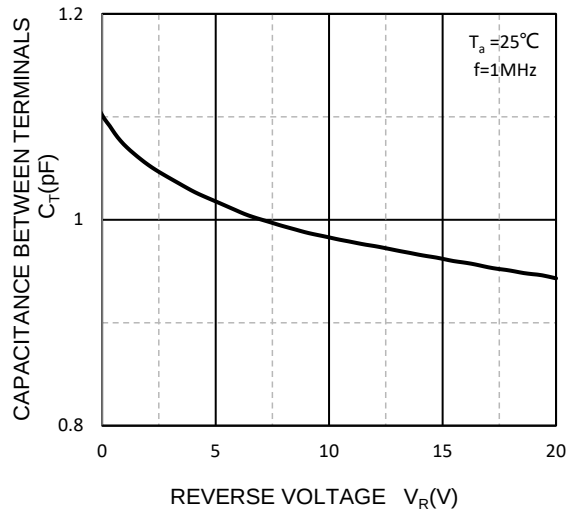
Capacitance Characteristics
