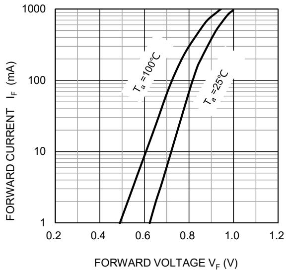
Forward Characteristics
