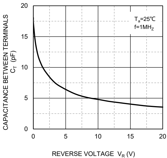
Capacitance Characteristics
