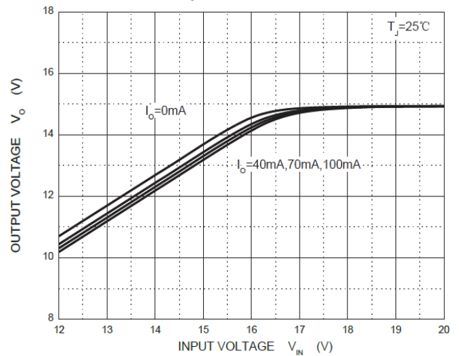
Dropout Characteristics
