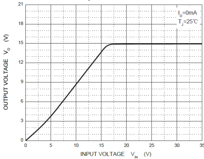
Output Characteristics
