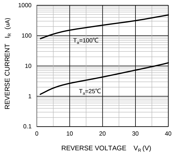
Reverse Characteristics
