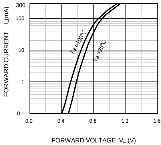
Forward Characteristics
