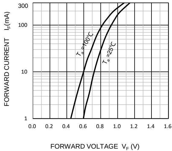
Forward Characteristics
