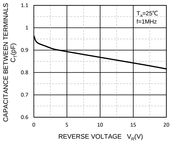
Capacitance Characteristics
