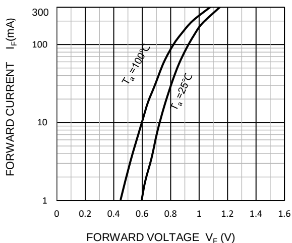
Forward Characteristics
