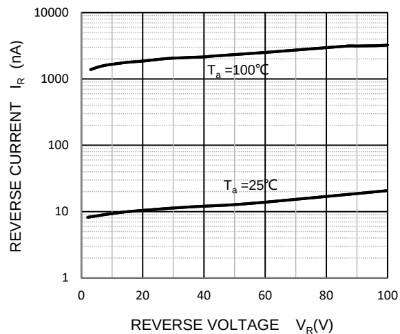
Reverse Characteristics
