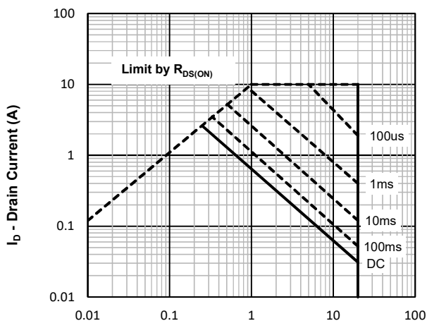
Fig5. Maximum Safe Operating Area
