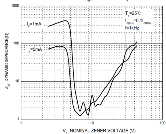
Effect of Zener Voltage on Zener Impedance
