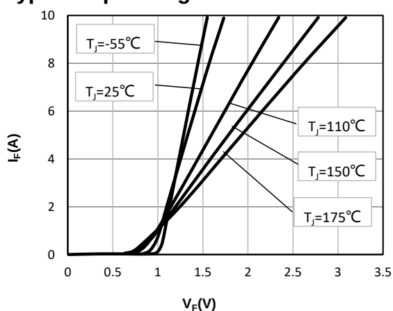
Fig1. Forward Characteristics
