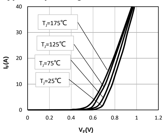
Fig1. Forward Characteristics
