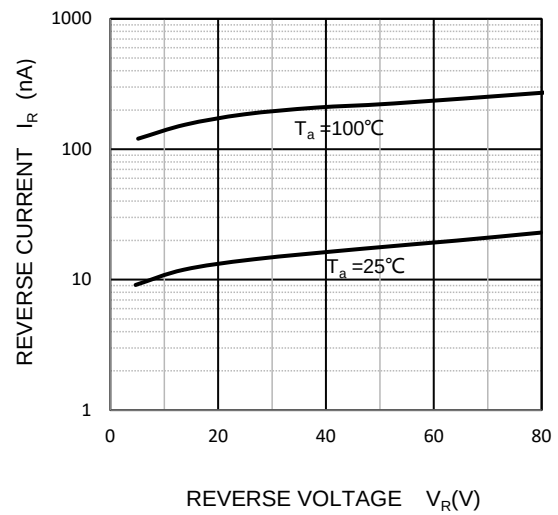
Reverse Characteristics
