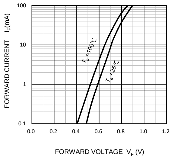
Forward Characteristics
