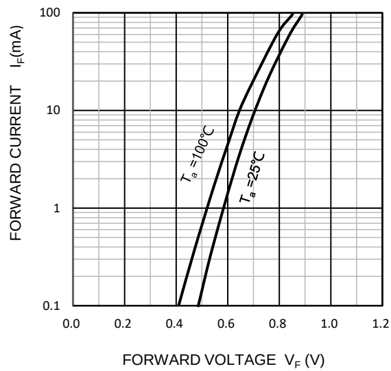
Forward Characteristics
