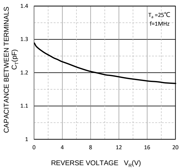
Capacitance Characteristics
