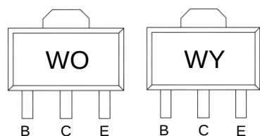
70-140 120-240 Marking and pin assignment
