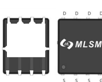
PDFN5X6-8L view
