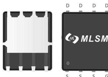
PDFN5X6-8L view
