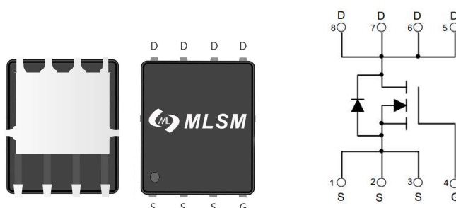
PDFN5X6-8L view
