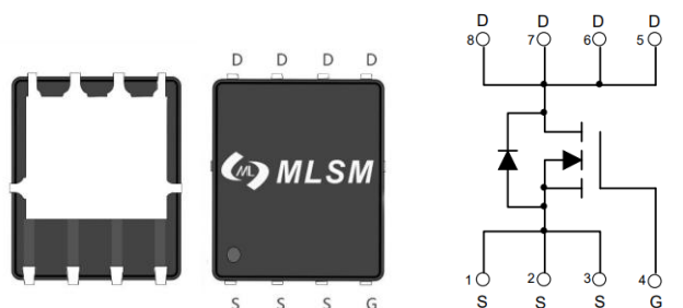
PDFN5X6-8L view
