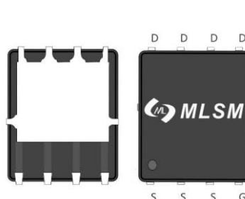
PDFN5X6-8L view
