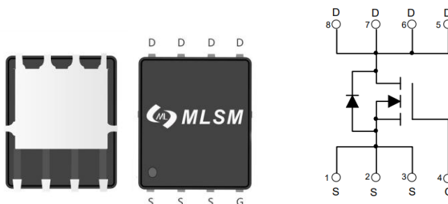
PDFN5X6-8L view
