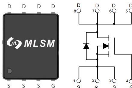
PDFN5X6-8L view
