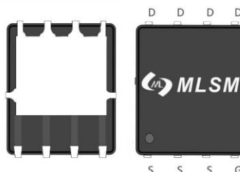
PDFN5X6-8L view
