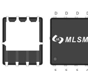
PDFN5X6-8L view
