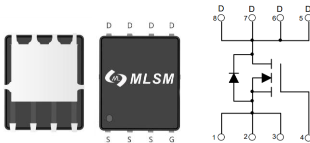
PDFN5X6-8L top view
