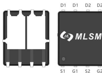
PDFN5X6-8L view
