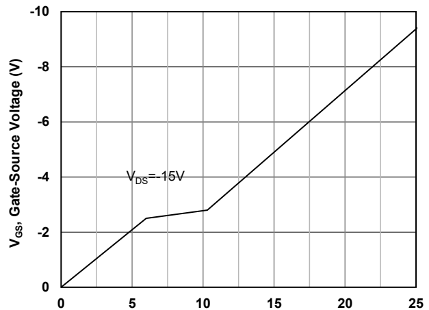
Q_g -Total Gate Charge (nC) Fig2. Typical Gate Charge Vs. Gate-Source Voltage
