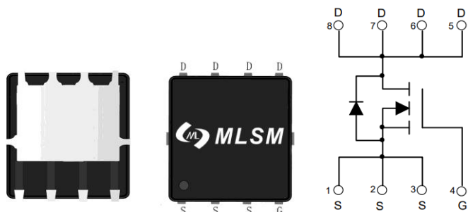
PDFN3X3-8L view
