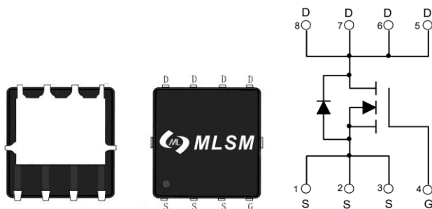
PDFN3X3-8L view
