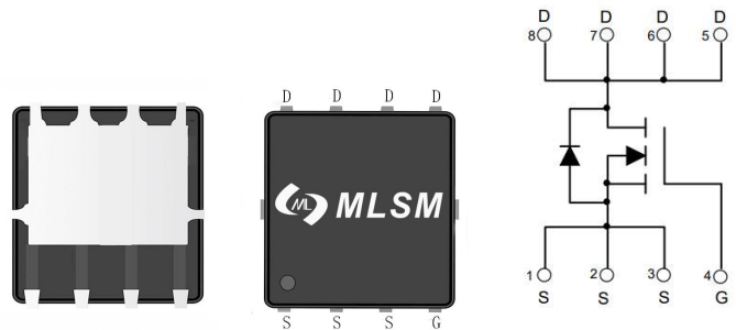
PDFN3X3-8L view
