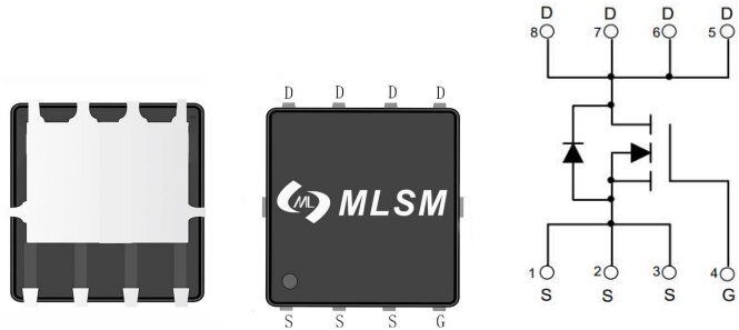
PDFN3X3-8L view
