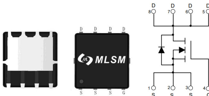
PDFN3X3-8L view
