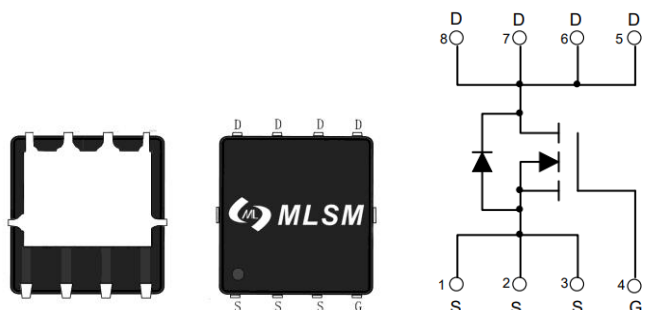
PDFN3X3-8L view
