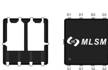
PDFN3X3-8L view
