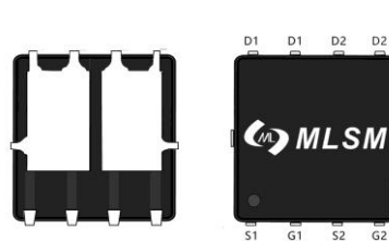
PDFN3X3-8L view
