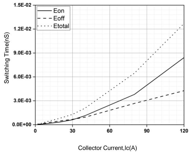
Figure 12. Typical switching energy losses as a function
