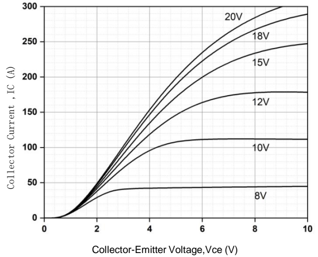
Figure 4. Typical output characteristic (Tj=150°C)
