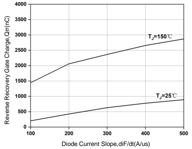
Figure 20. Typical reverse recovery time as a function of diode current slope ( V_{CC}=400V , I_F=40A )
