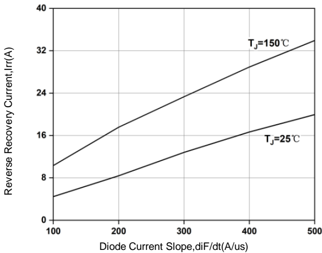
Figure 21. Typical reverse recovery current as a function of diode current slope ( V_{CC}=400V , I_F=40A )
