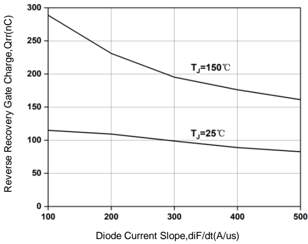
Figure 19. Typical reverse recovery charge as a function of diode current slope ( V_{CC}=400V , I_F=40A )
