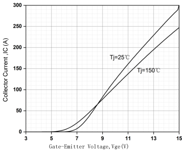
Figure 5. Typical transfer characteristic (Vce=20V)
