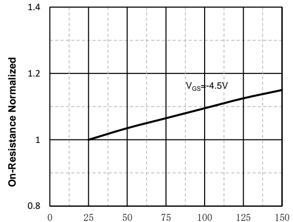
T_j - Junction Temperature ( ^{\circ}C ) Fig4. Normalized On-Resistance Vs. Temperature
