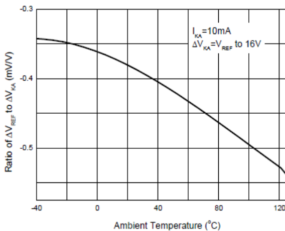
Ratio of Delta Reference Voltage to the Ratio of Delta Cathode Voltage vs. Ambient Temperature
