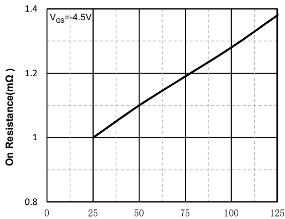
Fig3. Drain-Source on Resistance
