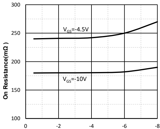
Fig3. On Resistance Vs. Drain-Source Current
