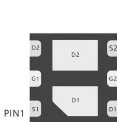
DFN2X2-6L view
