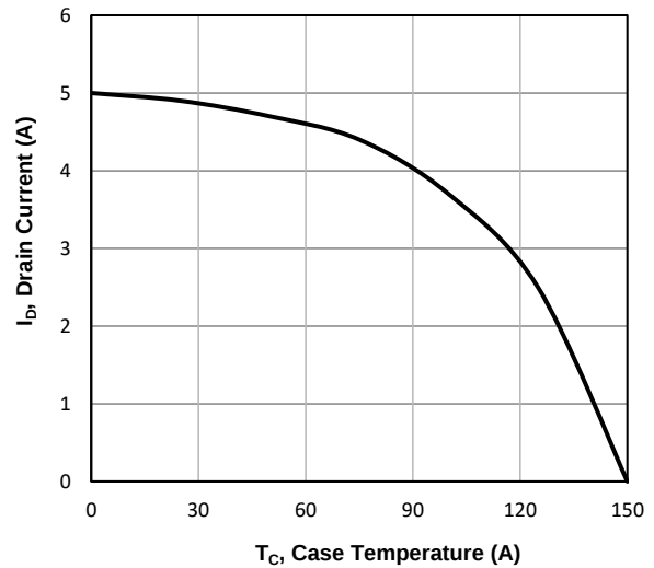
Fig4. Drain Current vs. Temperature
