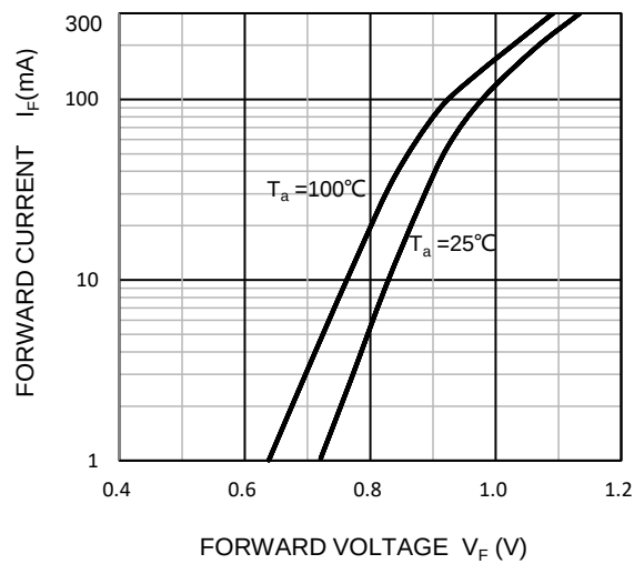
Forward Characteristics
