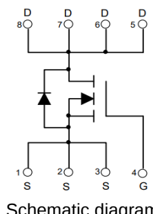
Schematic diagram
