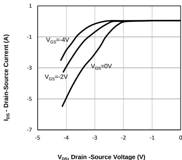
Fig5. Body Diode Characteristics
