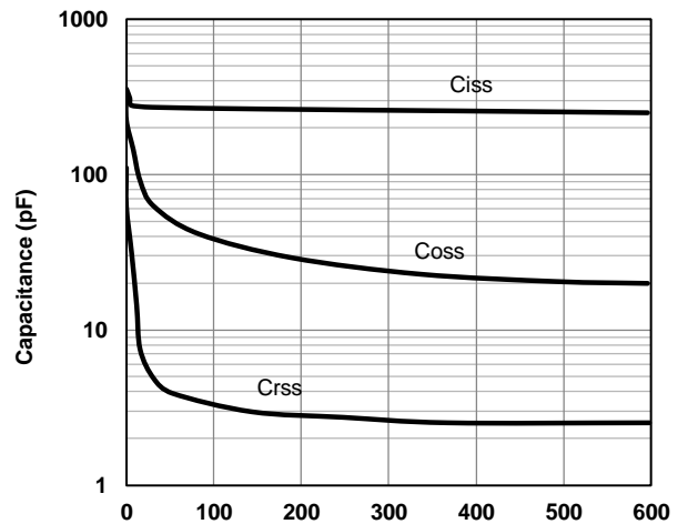
Fig6 Typical Capacitance Vs. Drain-Source
