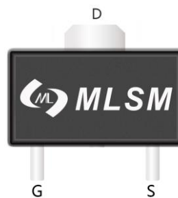
SOT-89-2L top view
