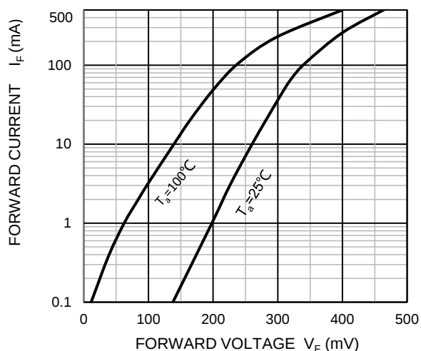
Forward Characteristics
