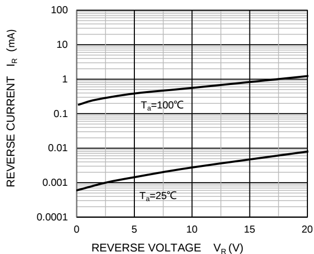
Reverse Characteristics
