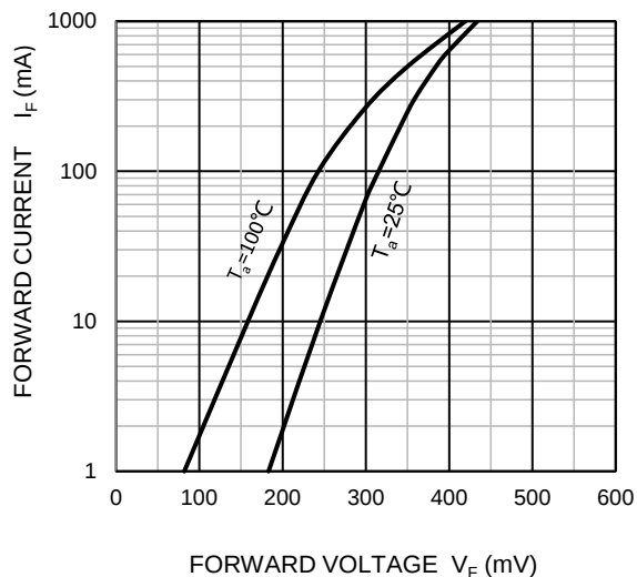
Forward Characteristics
