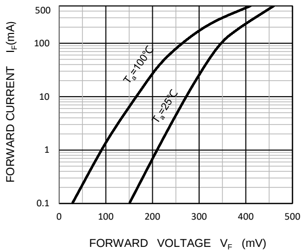
Forward Characteristics
