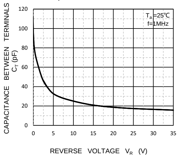
Capacitance Characteristics
